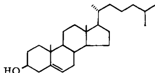
Cholesterin
