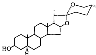
Tigogenin
